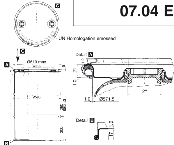
This example shows an open head, composite drum 205 liters
