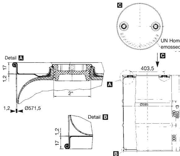
This example shows a composite drum 205 liters
